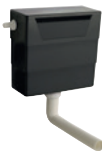
Universal Access Dual Flush Concealed WC Cistern H310 x W335 x D140mm Compatible with all WC Units Chrome Button XTY6T01 £90.00 Matt Black Button XTY6T02 £102.00 Brushed Brass Button XTY6T03 £102.00
