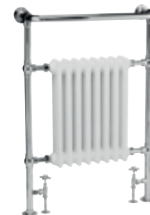
Harrow H965 x W673mm Chrome & White MTY022 £585.00 2252 Btu/hr
