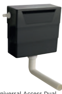
Universal Access Dual Flush Concealed WC Cistern H310 x W335 x D140mm Compatible with all WC Units
